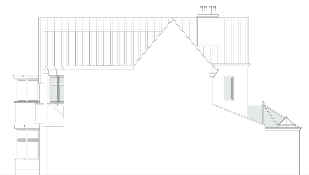
Proposed Side (south) Elevation 1:100 @ A1
