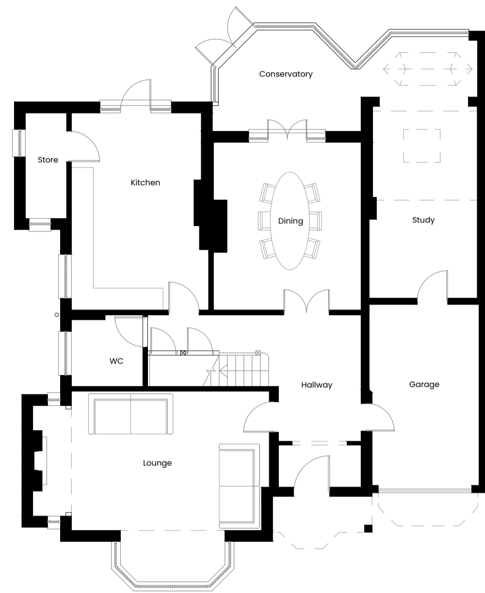
Existing Ground Floor Plan 1:100 @ A1
