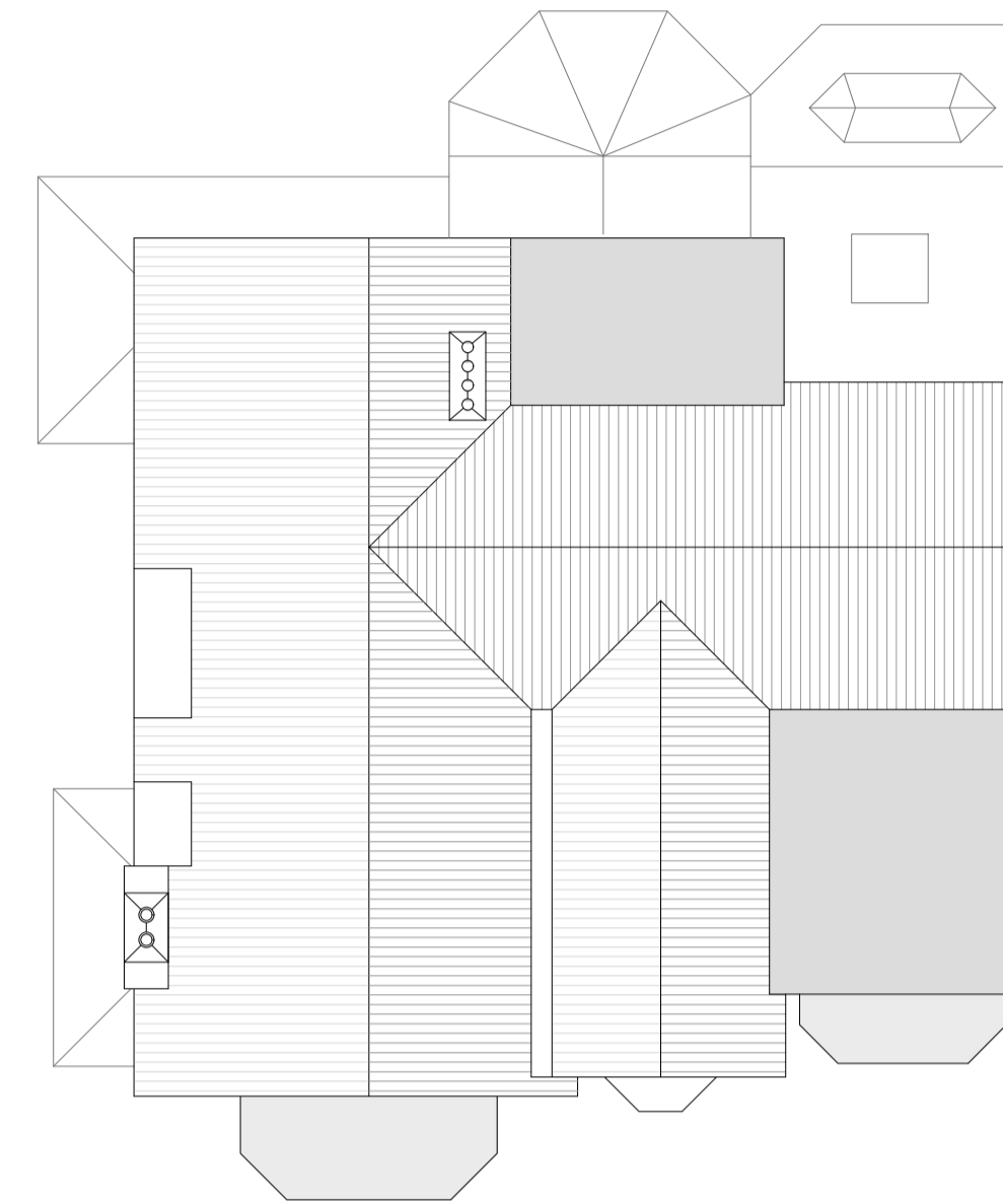
Existing Roof Plan 1:100 @ A1
