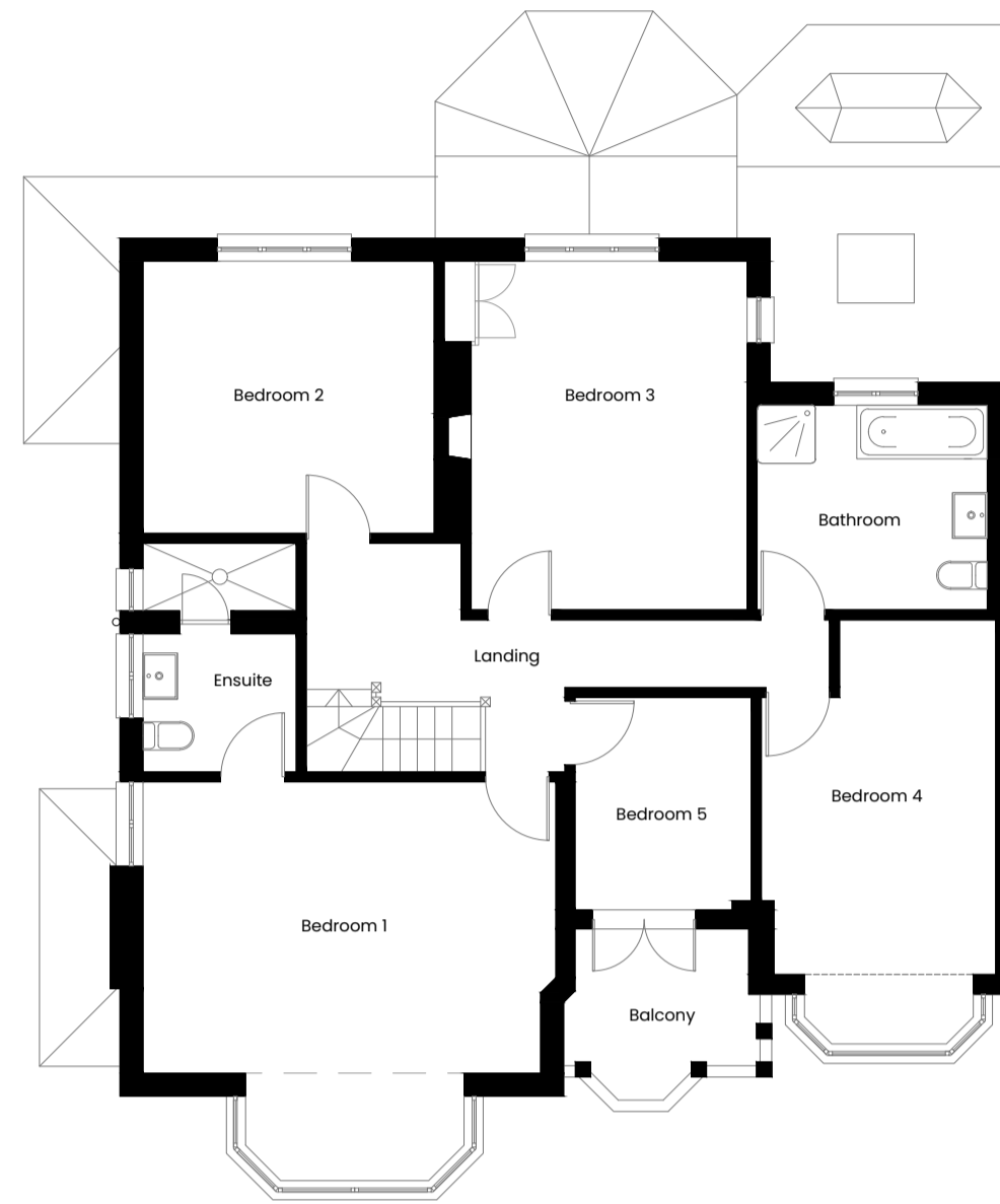
Existing First Floor Plan 1:100 @ A1
